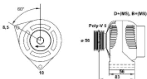
0633 41772 010 MAN214 75A 14V
