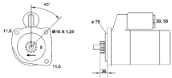
9432 41001 010 MSR1001 1,4Kw 12V
